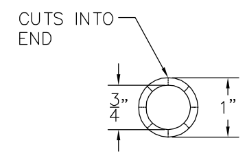
TYPICAL TAPER FOR 1" O.D ALIGNMENT PIN (END VIEW)
